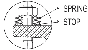
SPRING LOADED PACKING DETAIL
