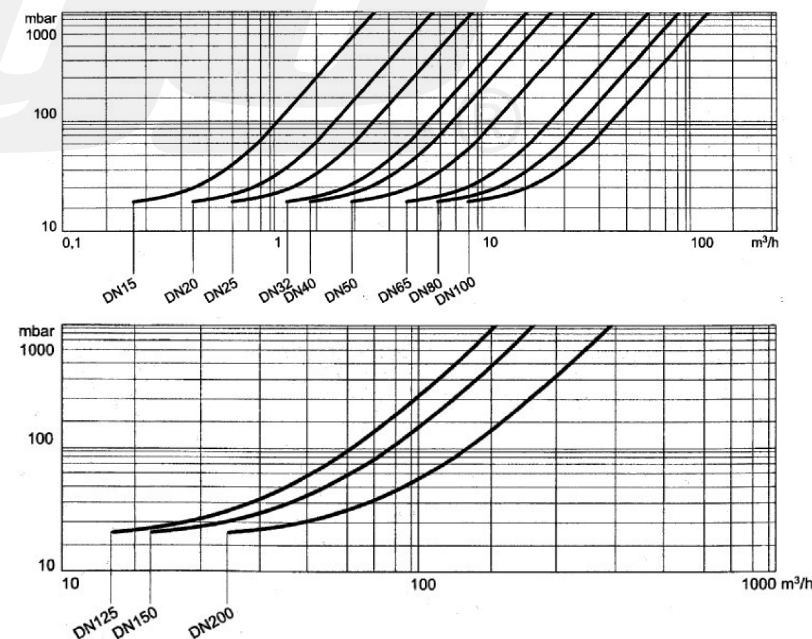
Diagramme de perte de pression / HEAD LOSSES DIAGRAM [H2O - 20°C, HORIZONTAL FLOW]
