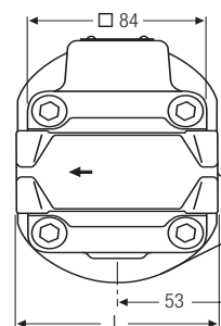
UNA 14h, with screwed sockets UNA 16h, with screwed sockets and socket-weld ends
