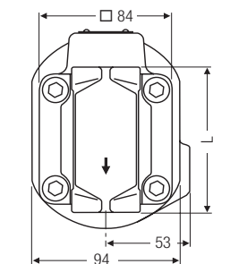
UNA 14v, with screwed sockets UNA 16v, with screwed sockets and socket-weld ends
