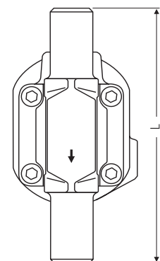
UNA 16v, with butt-weld ends
