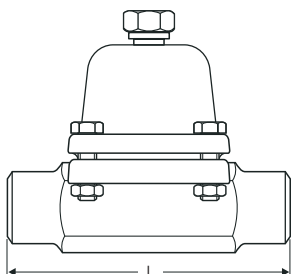
With butt-weld ends via transition pieces DN 40, 50
