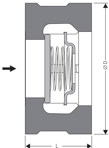
DN 15-100 Optional: with connection for electrostatic discharge line
